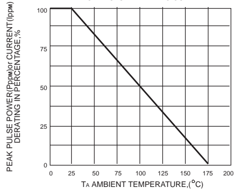
FIG. 2-PULSE DERATING CURVE
